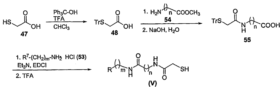
Scheme 7
